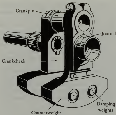
FIGURE 1-9. A single-throw radial engine crankshaft.
